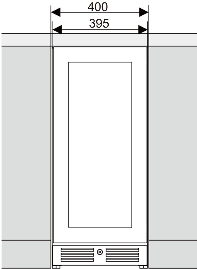
Front View
