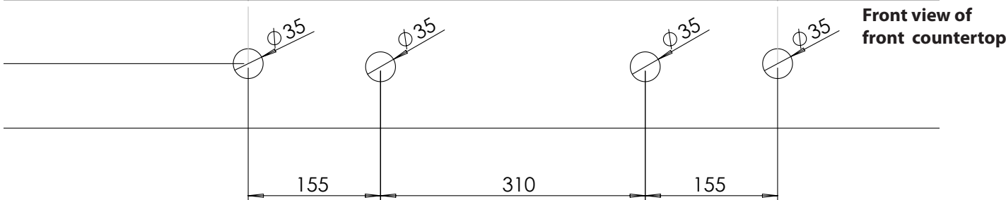
Hole pattern DXF file
